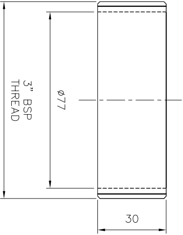
(SCALE-1:4) DETAIL-A BUSH FOR COUPLER
